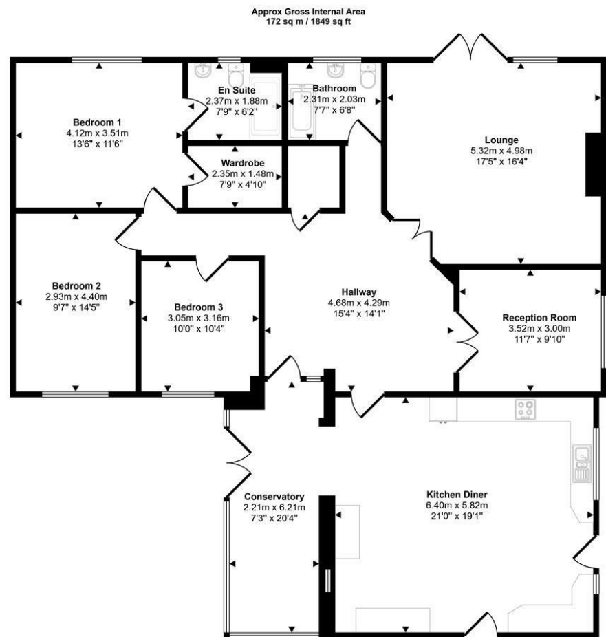
Floorplan
